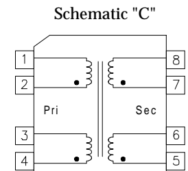
8-Pin Bottom View
