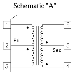
6-Pin Bottom View
